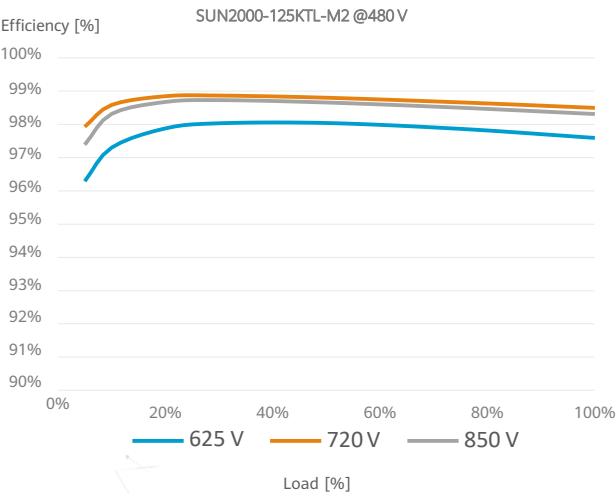
Efficiency Curve
